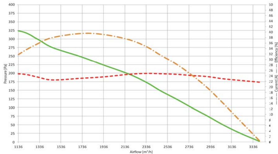
Axial fan performance curve
