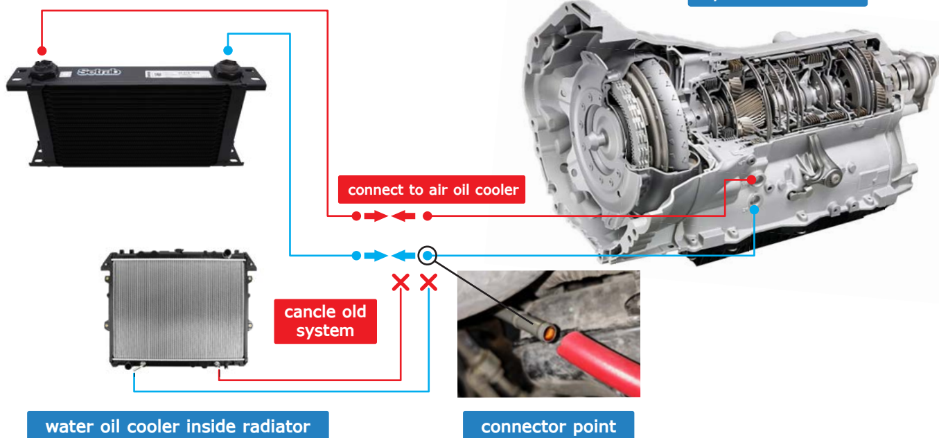
A/T Transmission
